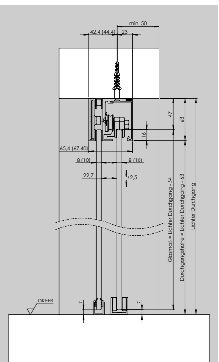
PLANE0 120, DECKENMONTAGE FÜR GLASANLAGEN CEILING MOUNTING FOR GLASS DOOR SYSTEM
